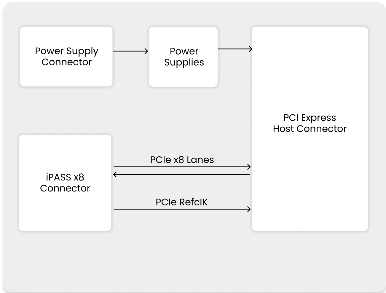
Figure 1 – ONIX-PCIE3-HOST-IPASS-8X Block Diagram
